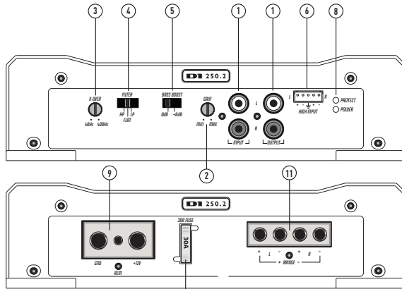
D1 250.2 2-Channel Amplifier
